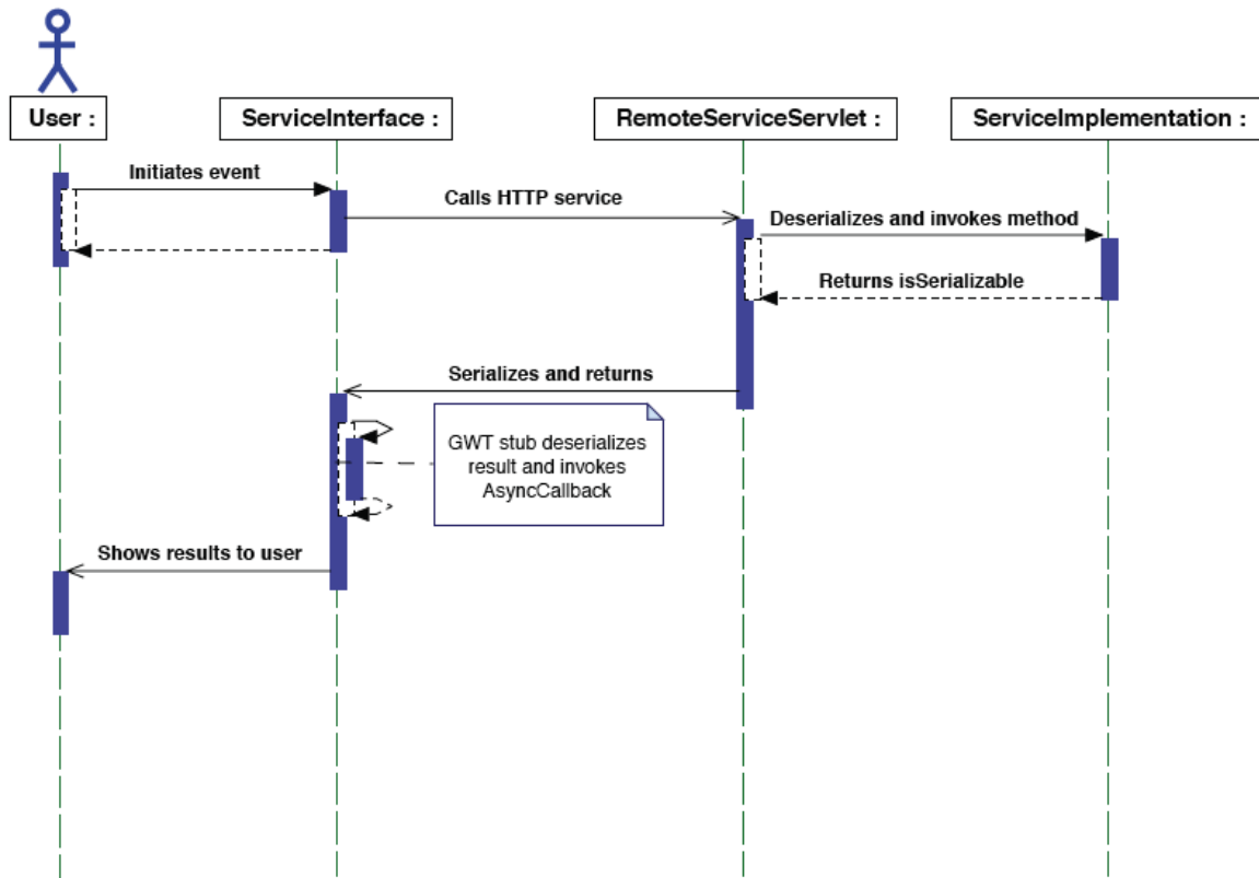
Figure 3.4 An overview of the complete RPC process. Notice that the user's browser lifeline is freed while the service call is executed; it's monopolized again as the call is returned.
